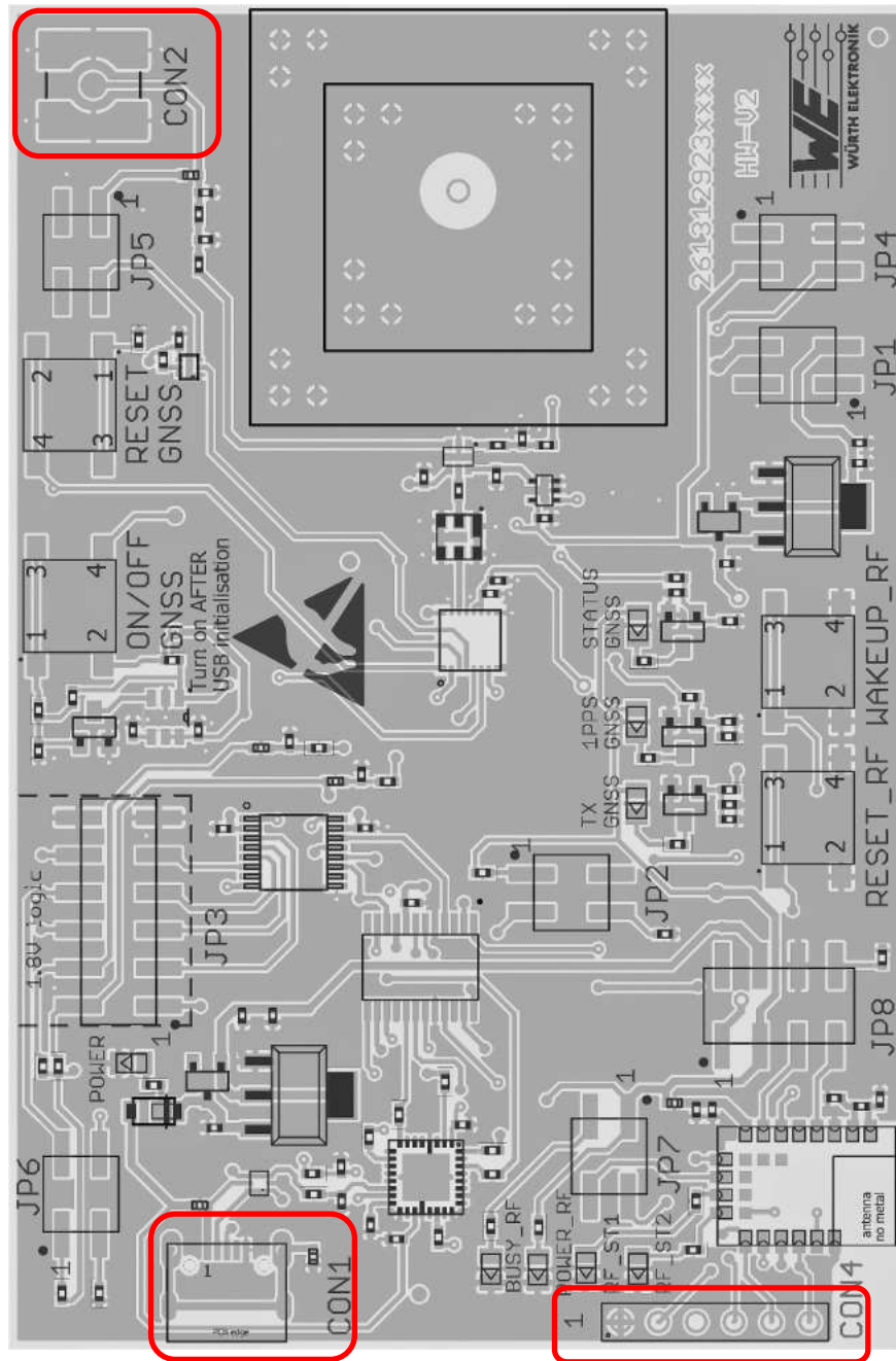
Figure 5: Connectors
