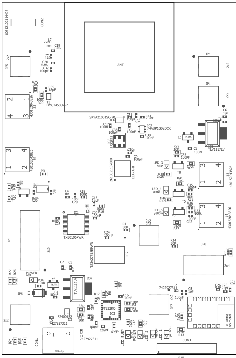
Figure 10: Assembly diagram
